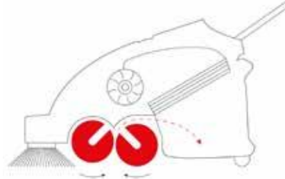
Tandem-Walzen-System (TRS)
